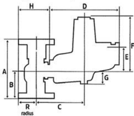
► Flanged Valve Body
